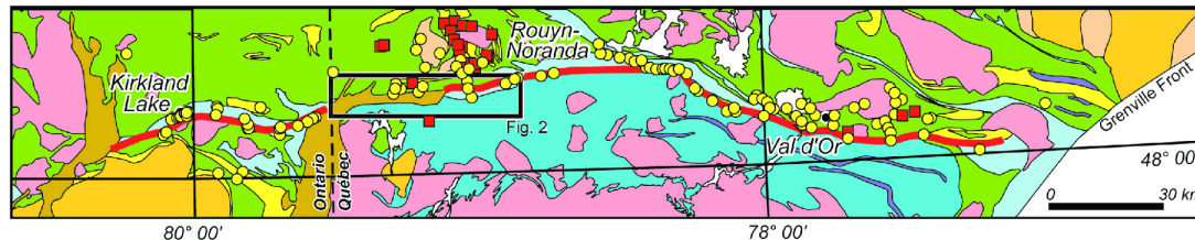
Figure Source: Rabeau et. al., 2011, Modified from Gold Potential of a Hidden Archean Fault Zone: The Case of the Cadillac-Larder Lake Fault, VL - 19, DO - 10.2113/gsemg.19.3-4.99, JO - Exploration and Mining Geology ER
